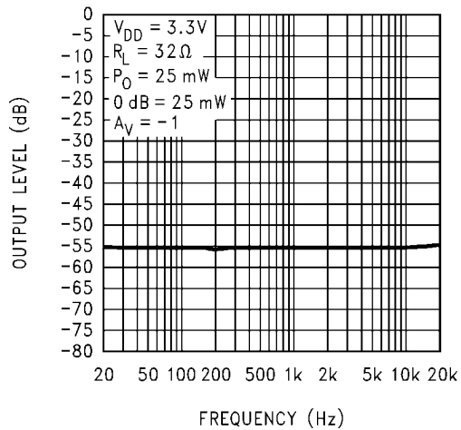
Channel Separation
