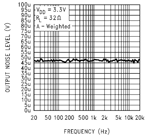
Noise Floor
