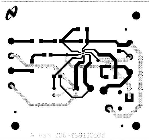
Composite View
