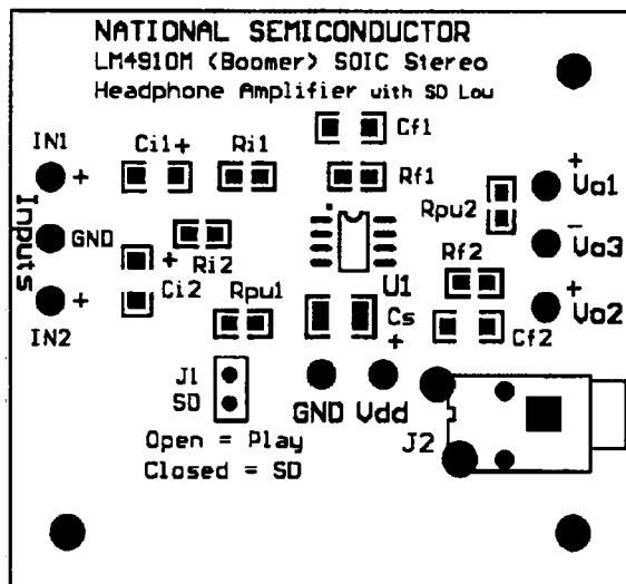
Silk Screen
