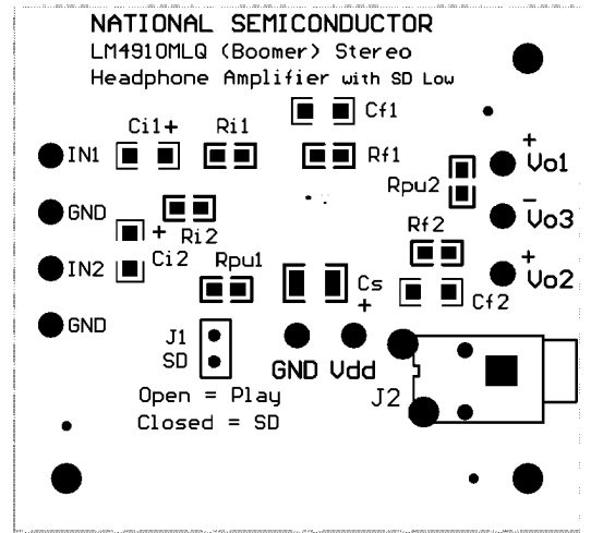
Silk Screen
