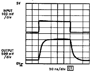
LM7131 Cable Driver A_V = +10 @ +5V
