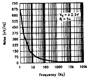
LM7131 Voltage Noise vs Frequency @ 5V
