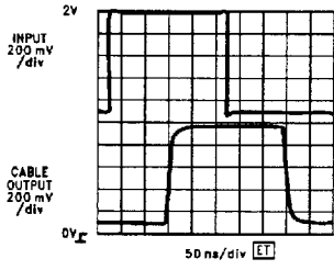
LM7131 Driving 75' RG-59 A_V = +2 @ +5V
