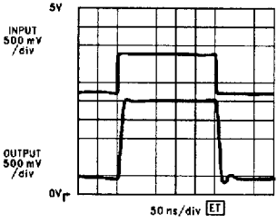
LM7131 Driving Flash A/D Load A_V = +2 @ +5V
