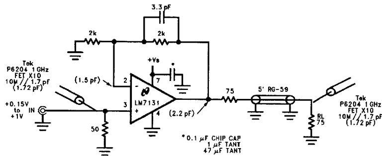
FIGURE 3. Cable Driver 5' RG-59
