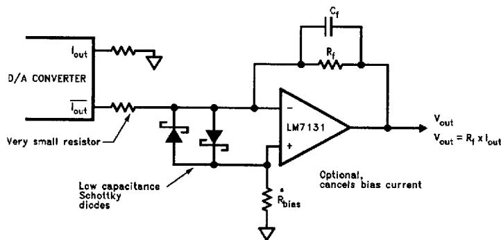
FIGURE 16. D/A Output Amplifier
