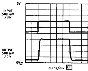
LM7131 Cable Driver A_V = +2 @ +5V
