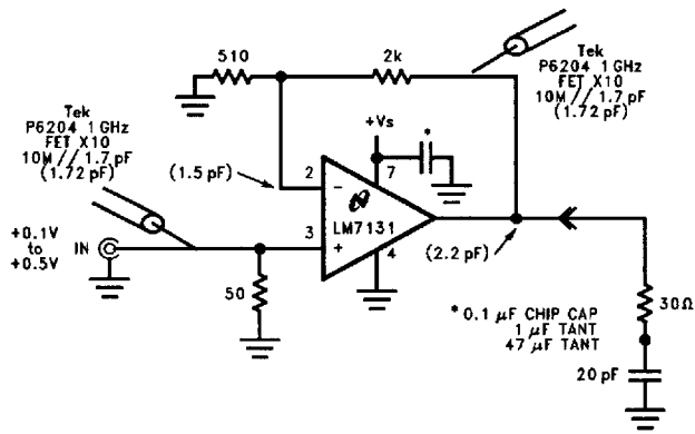
FIGURE 9. Flash A/D A_V = +5
