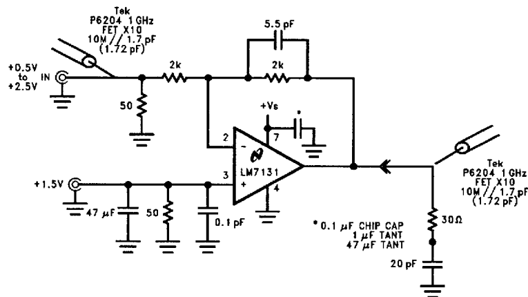
FIGURE 6. Flash A/D A_V = -1
