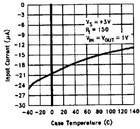
LM7131 Input Current vs Temperature @ 3V
