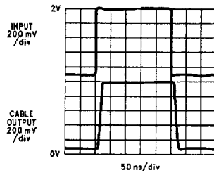
LM7131 Driving 5' RG-59 A_V = +2 @ +3V
