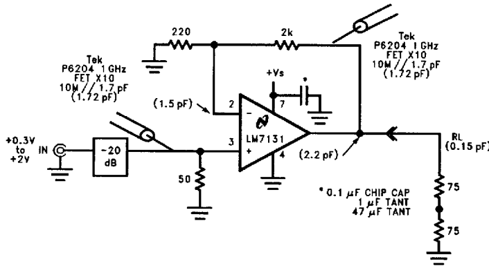
FIGURE 5. Cable Driver Gain of 10 A_v = +10
