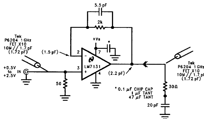
FIGURE 7. Flash A/D A_V = +1
