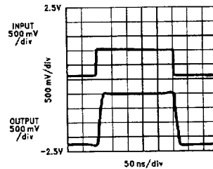
LM7131 Cable Driver A_V = +2 @ +3V
