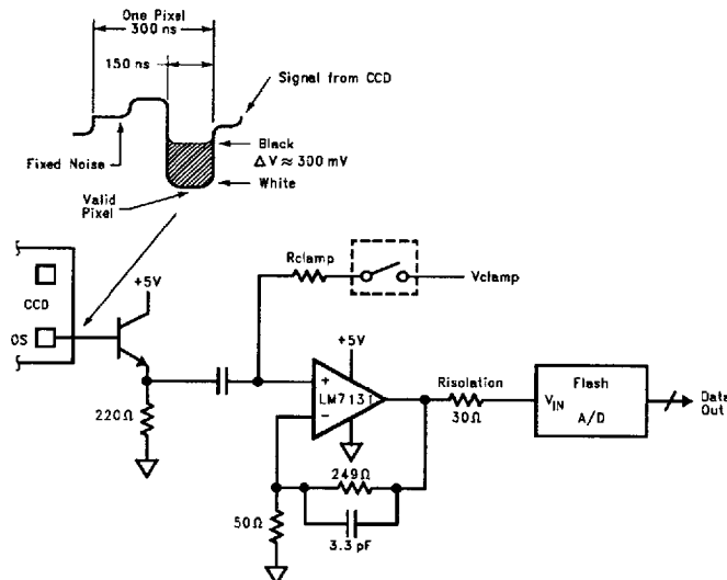
FIGURE 15. CCD Amplifier
