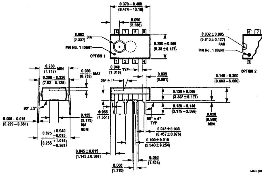
8-Pin Molded DIP 8-Lead (0.300" Wide) Molded Dual-In-Line Package Order Package Number LM7131ACN or LM7131BCN NS Package Number N08E
