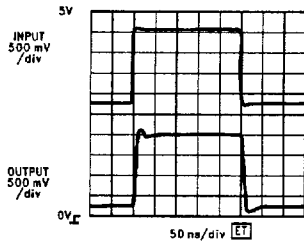
LM7131 Cable Driver A_V = +1 @ +5V
