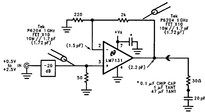
FIGURE 11. Flash A/D A_v = +10
