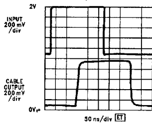
LM7131 Driving 75' RG-59 A_V = +2 @ +3V
