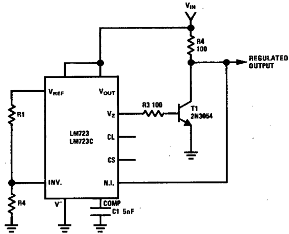
FIGURE 11. Remote Shutdown Regulator with Current Limiting
