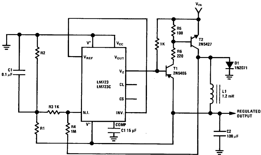
FIGURE 9. Positive Switching Regulator
