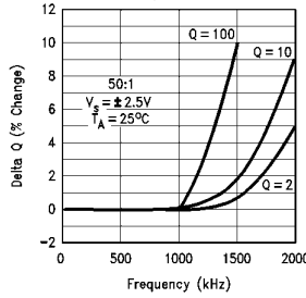
Q Deviation vs Clock Frequency
