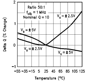
Q Deviation vs Temperature
