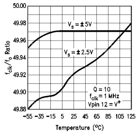
f_{CLK}/f_0 Ratio vs Temperature
