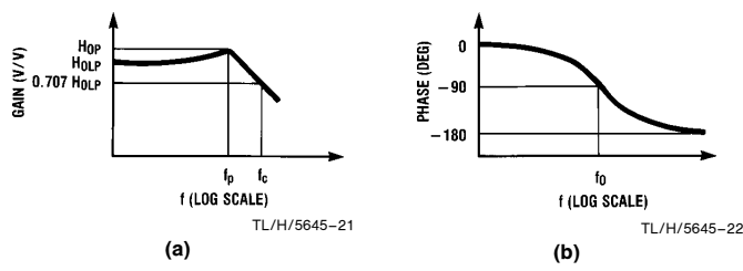
FIGURE 2. 2nd-Order Low-Pass Response
