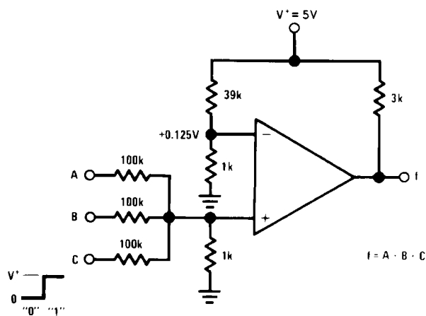
FIGURE 12. AND Gate
