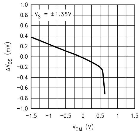
\Delta V_{OS} vs. CMR
