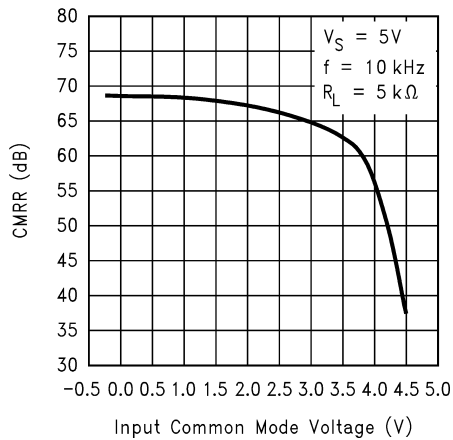
CMRR vs. Input Common Mode Voltage
