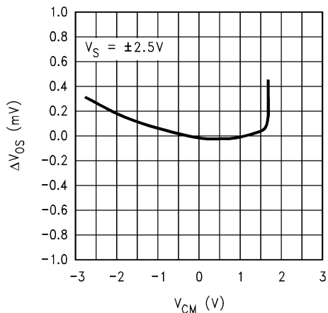
\Delta V_{OS} vs. CMR
