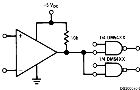
FIGURE 11. Driving TTL
