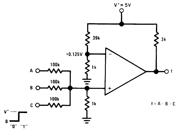
FIGURE 12. AND Gate
