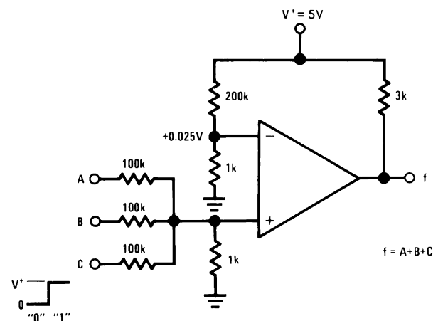
FIGURE 13. OR Gate
