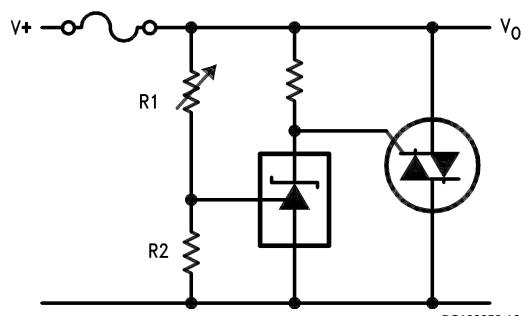
Crow Bar
