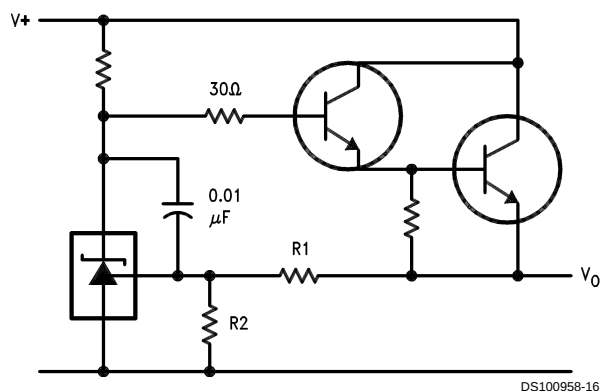
Series Regulator
