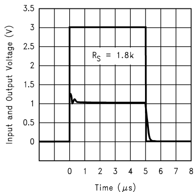
Pulse Response 2
