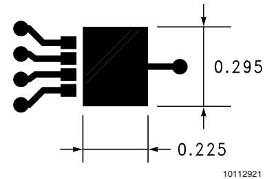
FIGURE 7. SCENARIO B, \theta_{JA} = 125^{\circ}\text{C}/\text{W}
