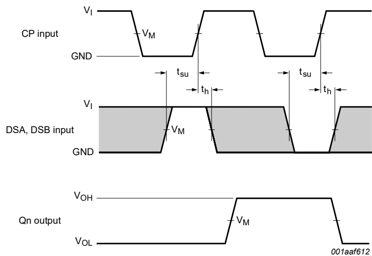
Measurement points are given in Table 8 . The shaded areas indicate when the input is permitted to change for predictable output performance. V_{\text{OL}} and V_{\text{OH}} are typical voltage output levels that occur with the output load.
