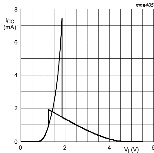
Fig. 10. Typical 74AHCT3G14-Q100 transfer characteristics
