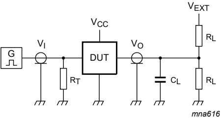
Fig. 12. Additional t_{pd} and t_{en} versus load capacitance
