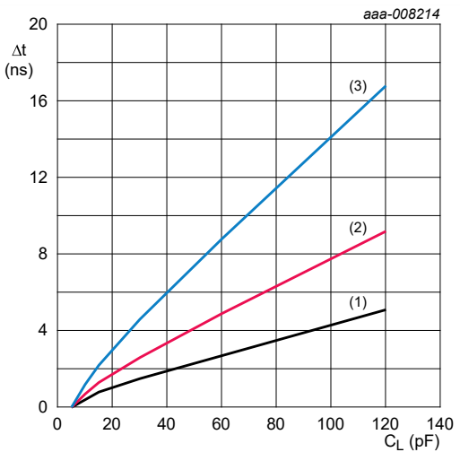
Fig. 9. Additional t_{pd} and t_{en} versus load capacitance
