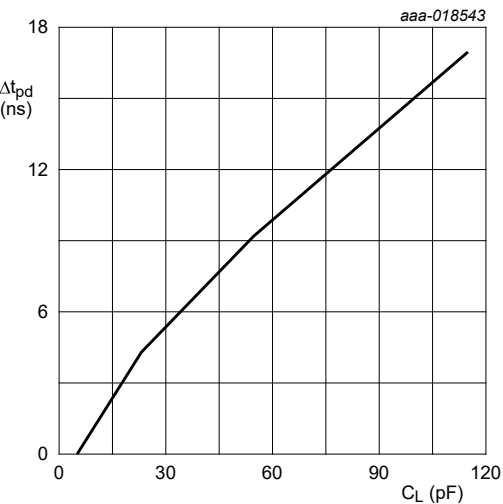
Fig. 21. Additional propagation delay versus load capacitance
