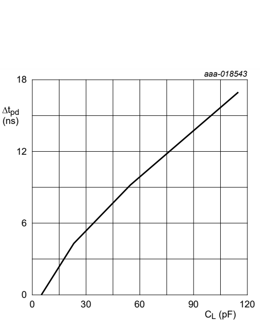
Fig. 10. Additional propagation delay versus load capacitance
