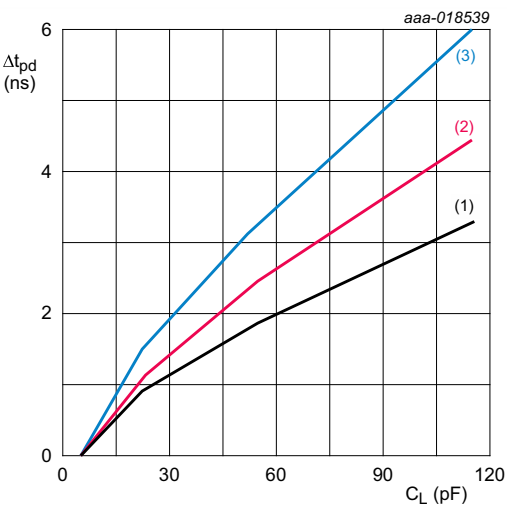
T_{amb} = -40\text{ }^{\circ}\text{C} to +85\text{ }^{\circ}\text{C} unless otherwise specified. For t_{PLH} , t_{PHL} and t_{PZL} (1) Minimum: V_{CCO} = 3.6\text{ V} (2) Typical: T_{amb} = 25\text{ }^{\circ}\text{C} ; V_{CCO} = 3.3\text{ V} (3) Maximum: V_{CCO} = 3\text{ V}
