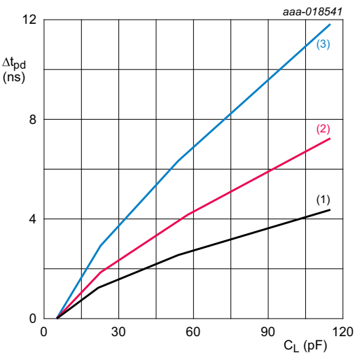
T_{amb} = -40\text{ }^{\circ}\text{C} to +85\text{ }^{\circ}\text{C} unless otherwise specified. For t_{PLH} , t_{PHL} and t_{PZL} (1) Minimum: V_{CCO} = 1.95\text{ V} (2) Typical: T_{amb} = 25\text{ }^{\circ}\text{C} ; V_{CCO} = 1.8\text{ V} (3) Maximum: V_{CCO} = 1.65\text{ V}
