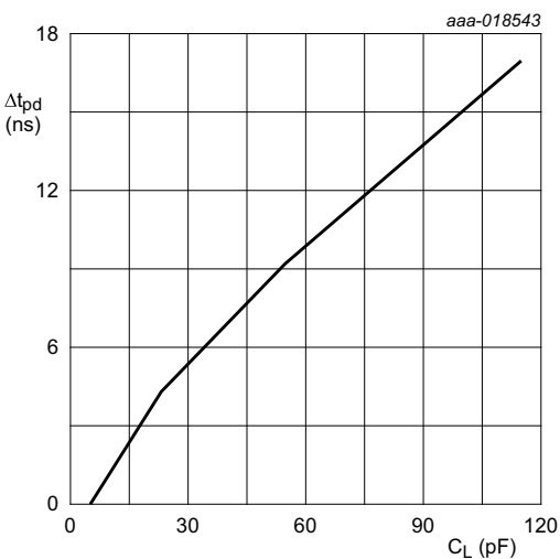
T_{amb} = 25 °C; V_{CCO} = 1.2 V. For t_{PLH} , t_{PHL} and t_{PZL}
