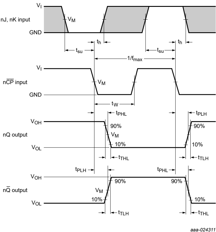
Measurement points are given in Table 8 . V_{OL} and V_{OH} are typical voltage output levels that occur with the output load. Fig. 4. Clock propagation delays, output transition time, pulse width, set-up, hold times, and maximum frequency
