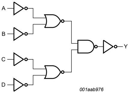
Fig. 4. Logic diagram
