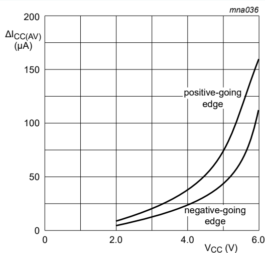
Fig. 11. \Delta I_{\text{CC(AV)}} as a function of V_{\text{CC}} for 74HC2G14
