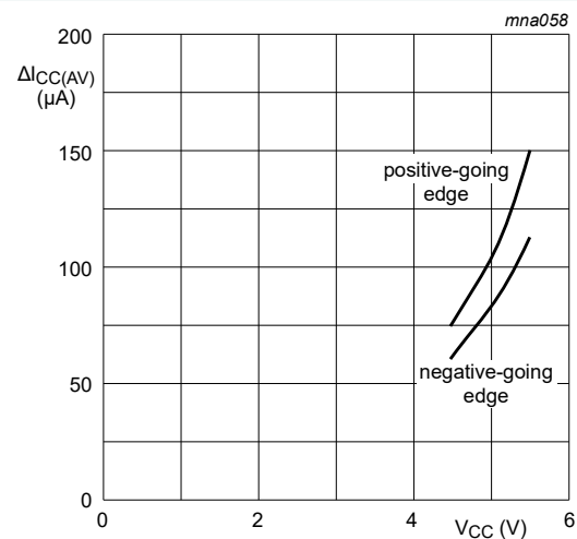
Fig. 12. \Delta I_{\text{CC(AV)}} as a function of V_{\text{CC}} for 74HCT2G14
