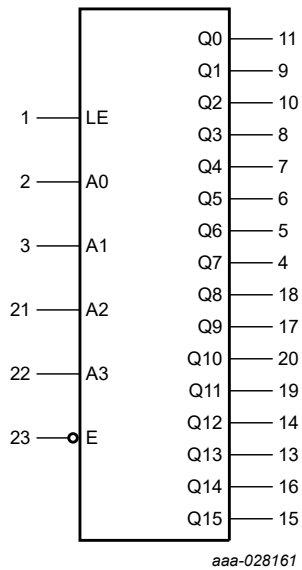
Fig. 1. Logic symbol
