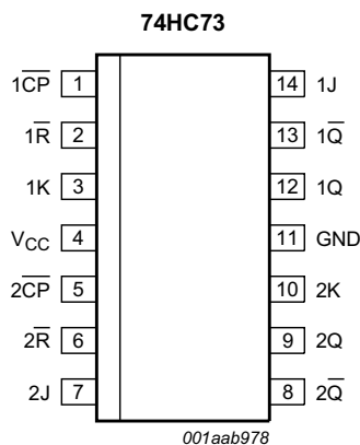
Fig 5. Pin configuration SO14, SSOP14 and TSSOP14
