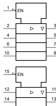
Fig. 2. IEC logic symbol
