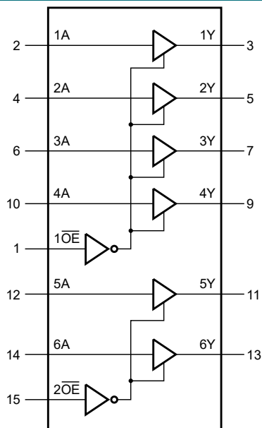
Fig. 1. Logic symbol
