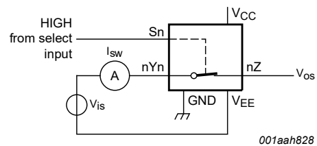
Fig. 10. Test circuit for measuring ON-state current
