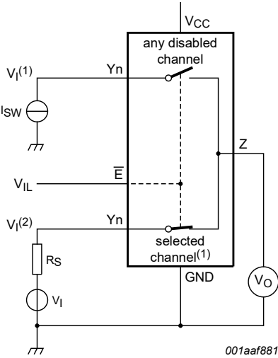
Fig. 5. Test circuit for measuring ON-state leakage current
