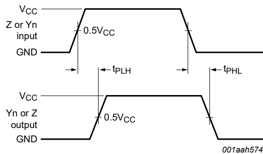
Fig. 8. Input (Z, Y n ) to output (Y n , Z) propagation delays
