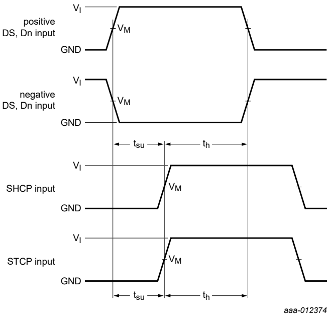
Fig. 9. Input MR to shift clock SHCP and storage clock STCP recovery times
