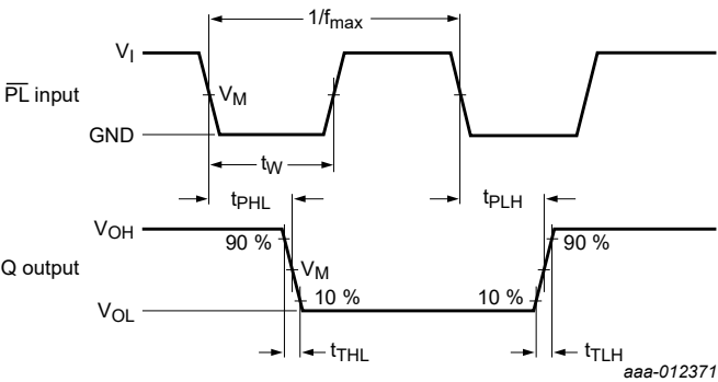
Fig. 8. Input PL to Q output propagation delays, PL pulse width and output transition times
