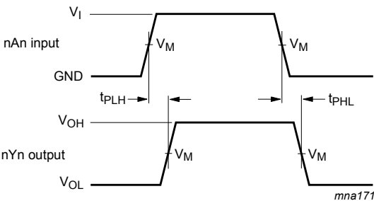
Fig. 5. Input nAn to output nYn propagation delays
