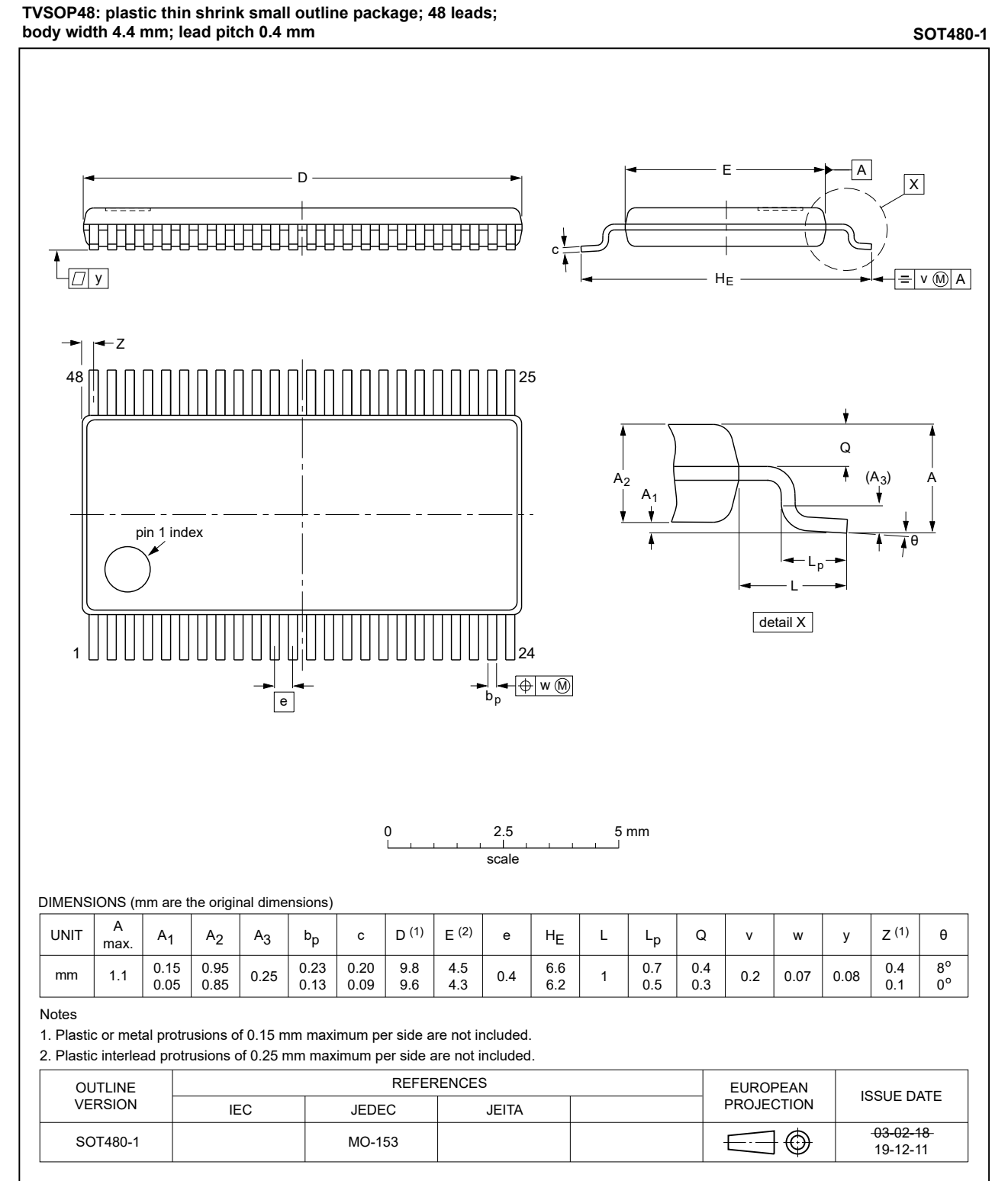
Fig. 8. Package outline SOT480-1 (TVSOP48)
