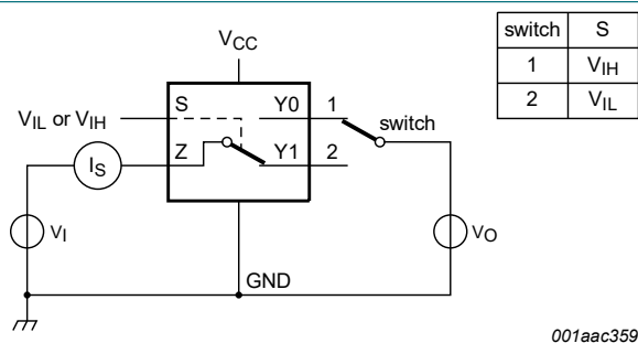
Fig. 3. Test circuit for measuring OFF-state leakage current
