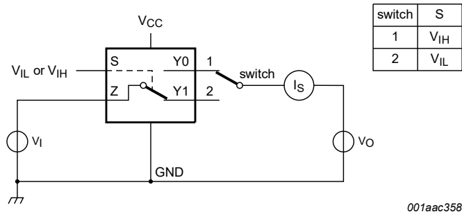
Fig. 3. Test circuit for measuring OFF-state leakage current
