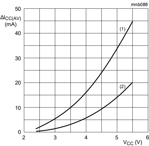
Linear change of V_I between 0.8 V to 2.0 V. All values given are typical unless otherwise specified. (1) Positive-going edge. (2) Negative-going edge.
