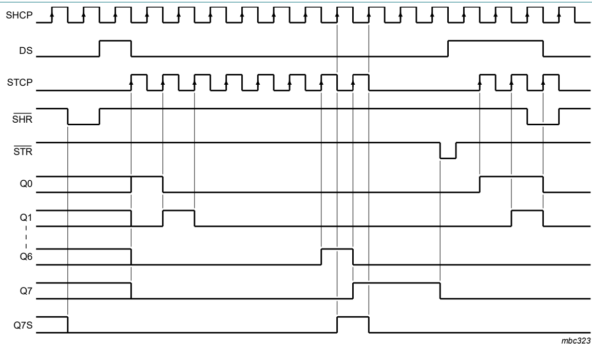
Fig. 4. Timing diagram
