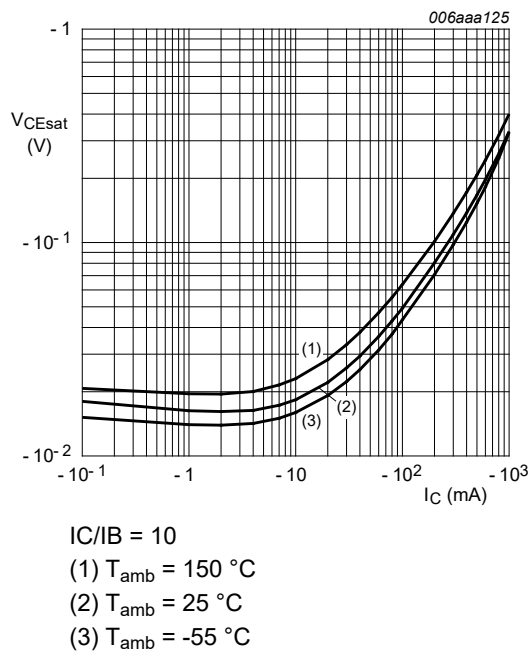
Fig. 6. BC807-16W: Collector-emitter saturation voltage as a function of collector current; typical values
