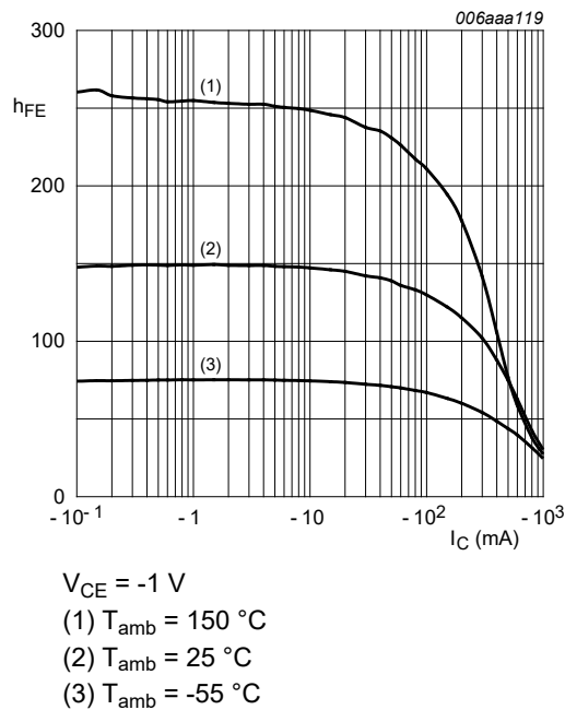
Fig. 4. BC807-16W: DC current gain as a function of collector current; typical values
