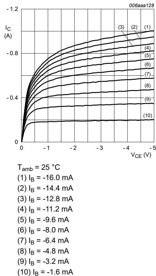
Fig. 7. BC807-16W: Collector current as a function of collector-emitter voltage; typical values
