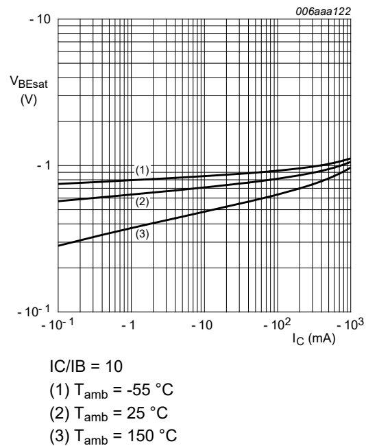
Fig. 5. BC807-16W: Base-emitter saturation voltage as a function of collector current; typical values
