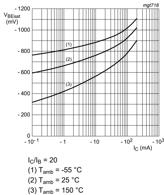
Fig. 9. BC857BW: Base-emitter saturation voltage as a function of collector current; typical values
