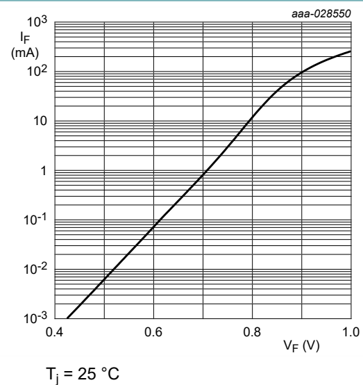
Fig. 2. BZX884-B/C2V4: Forward current as a function of forward voltage; typical values
