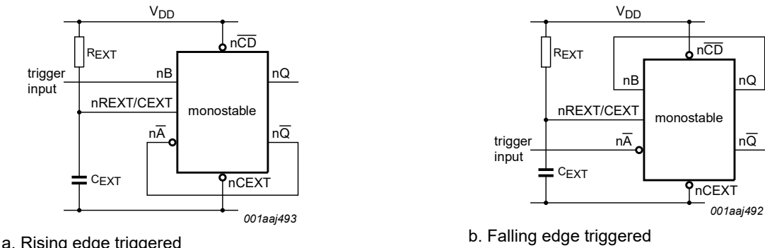
Fig. 7. Non-retriggerable applications
