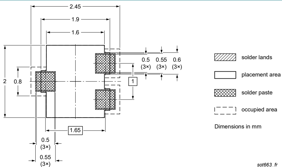
Fig. 9. Reflow soldering footprint for SOT663
