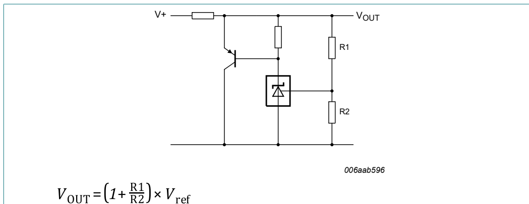
Fig. 24. High-current shunt regulator
