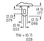
Solder Lug (W01)
