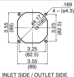
INLET SIDE / OUTLET SIDE
