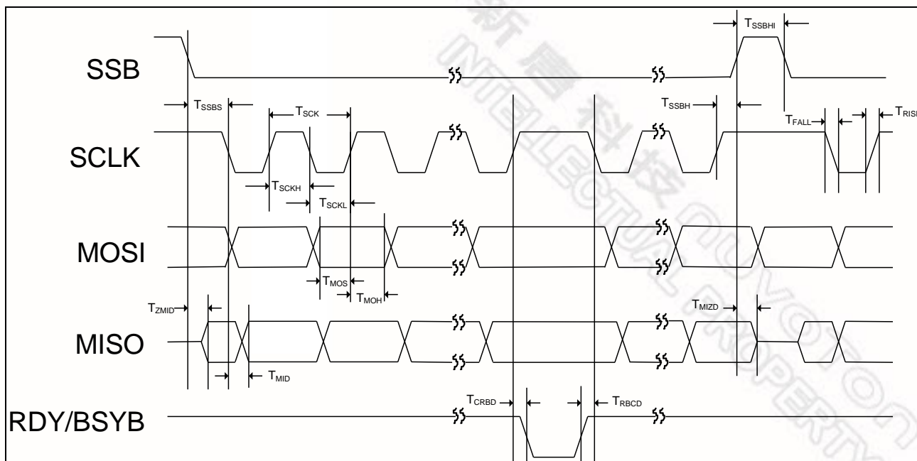
Figure 12-1 SPI Timing
