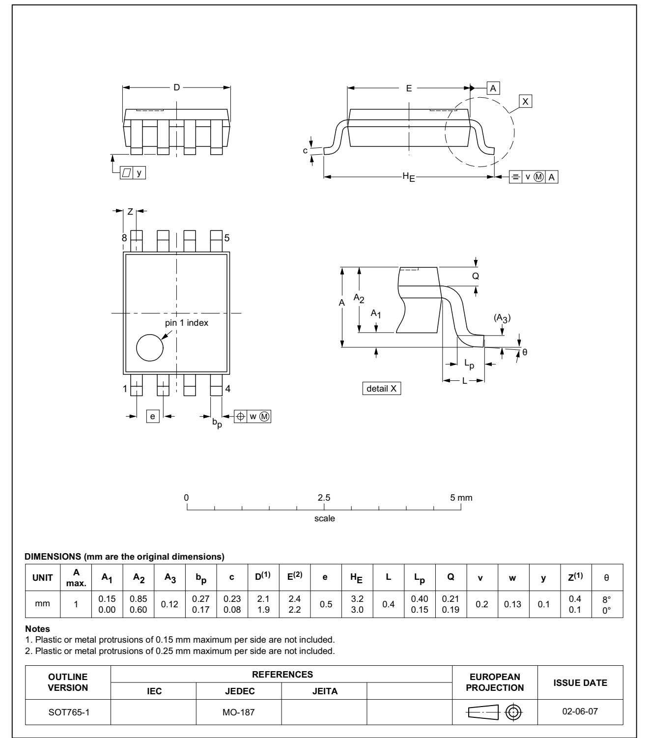
Fig 8. Package outline SOT765-1 (VSSOP8)
