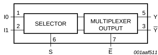
Fig 3. Logic diagram
