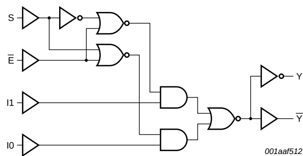
Fig 4. Functional diagram
