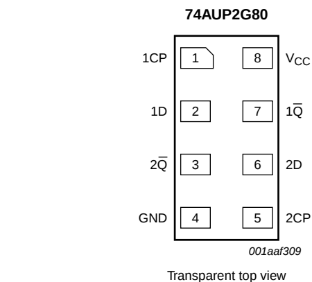
Fig 5. Pin configuration SOT833-1, SOT1089, SOT1116 and SOT1203
