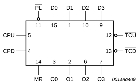
Fig 2. Logic symbol
