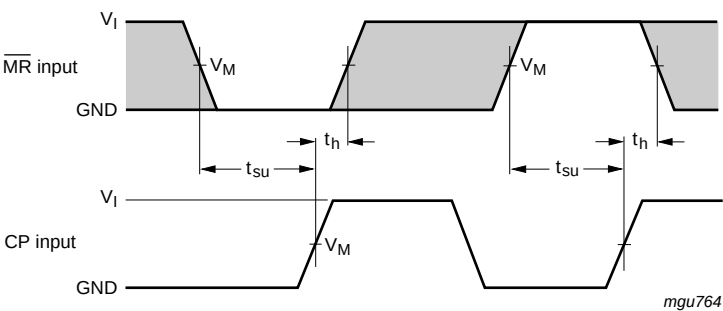
The shaded areas indicate when the input is permitted to change for predictable output performance.
