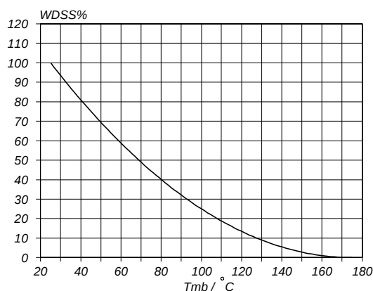
Fig.17. Normalised avalanche energy rating. W_{DSS}\% = f(T_{mb}) ; conditions: I_D = 75\text{ A}
