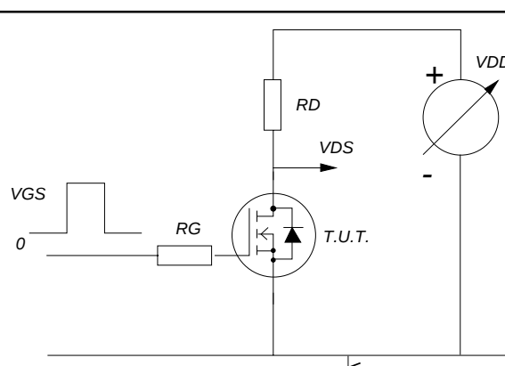
Fig.20. Switching test circuit.
