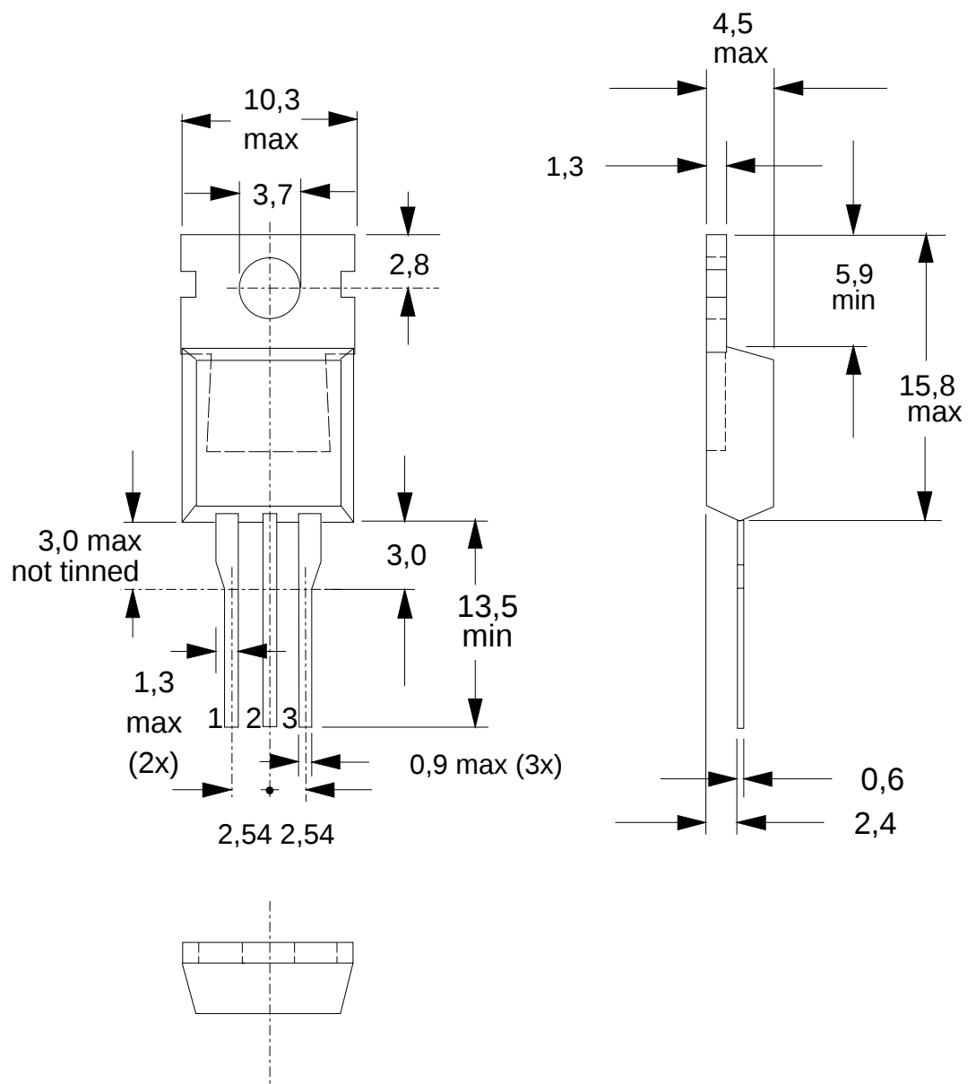
Fig.21. SOT78 (TO220AB); pin 2 connected to mounting base.
