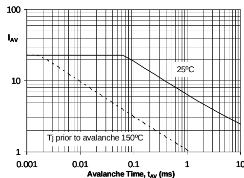
Fig.19. Maximum permissible repetitive avalanche current( I_{AV} ) versus avalanche time( t_{AV} ) for unclamped inductive loads.
