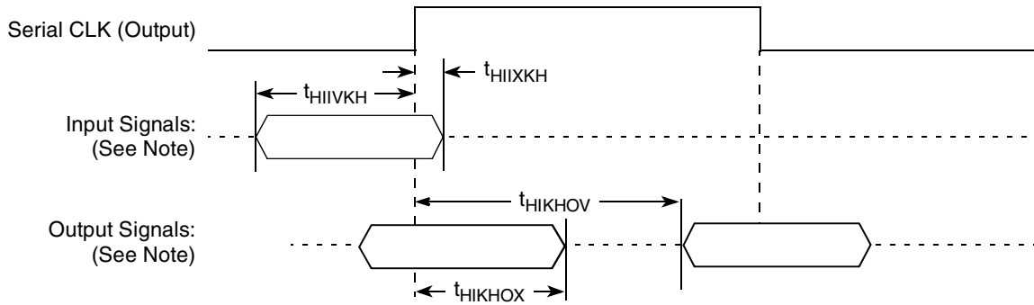
Figure 40. AC Timing (Internal Clock) Diagram
