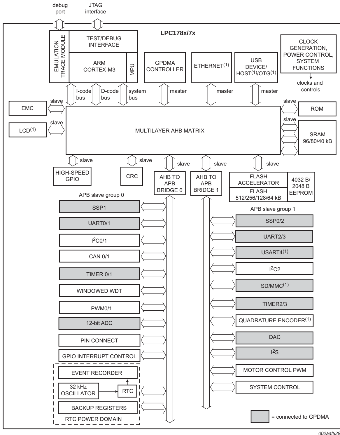
Fig 1. Block diagram
