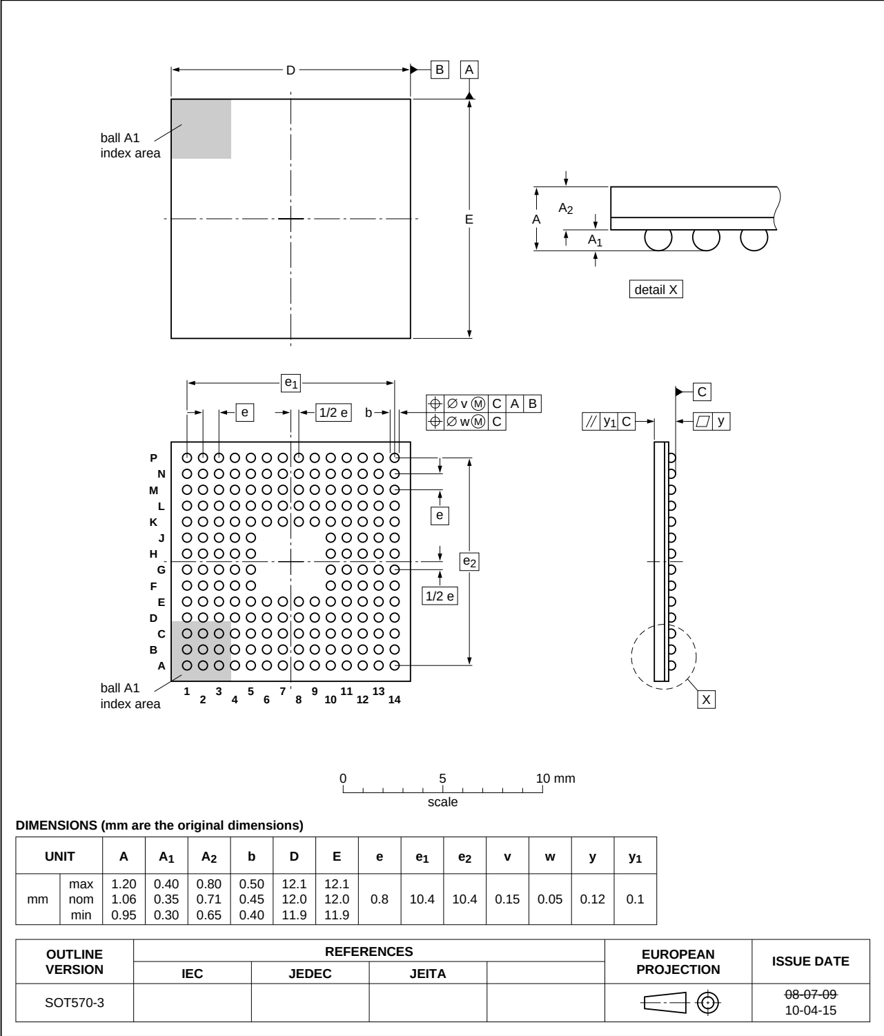
Fig 43. TFBGA180 package
