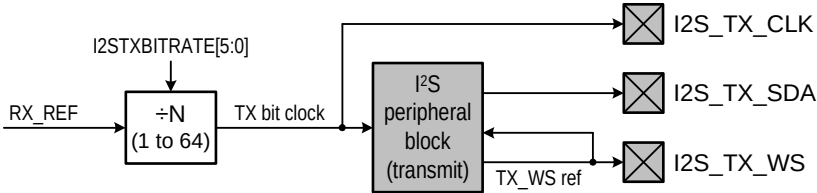
Fig 125. Transmitter master mode sharing the receiver reference clock
