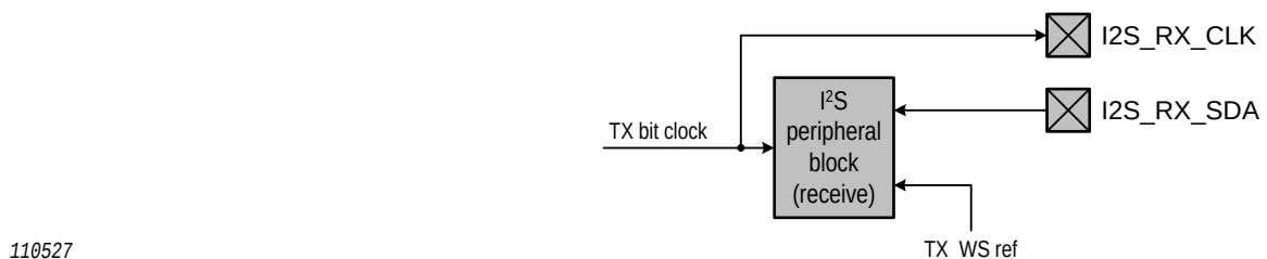
Fig 132. 4-wire receiver master mode sharing the transmitter bit clock and WS
