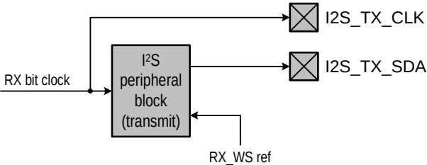
Fig 126. 4-wire transmitter master mode sharing the receiver bit clock and WS
