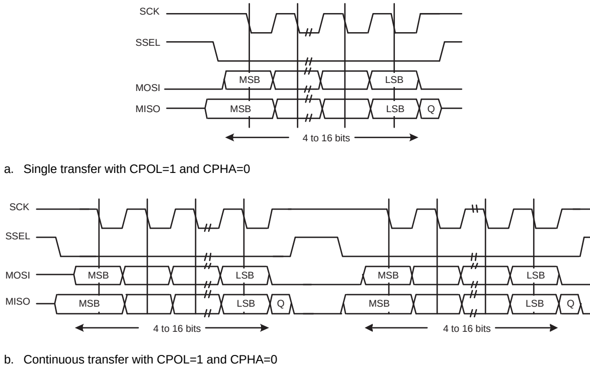
Fig 102. SPI frame format with CPOL = 1 and CPHA = 0 (a) Single and b) Continuous Transfer)
