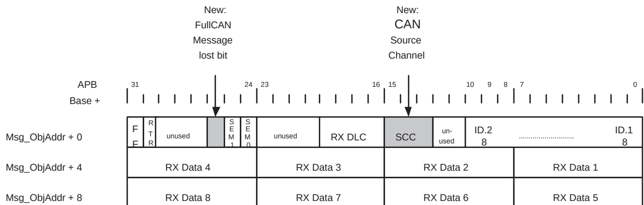
Fig 89. FullCAN message object layout
