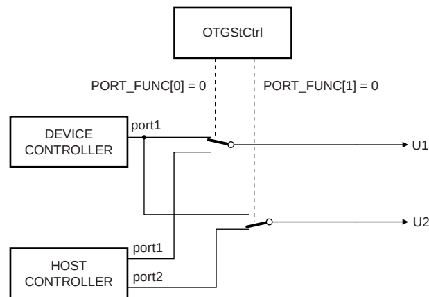
Fig 52. Port selection for PORT_FUNC bit 0 = 0 and PORT_FUNC bit 1 = 0
