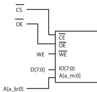
Fig 19. 8 bit bank external memory interface (bits MW = 00)
