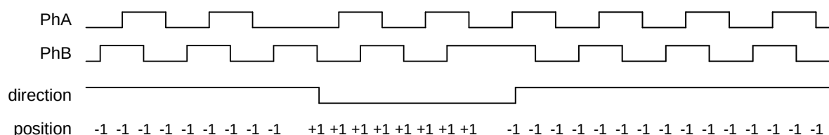
Fig 152.Quadrature Encoder Basic Operation
