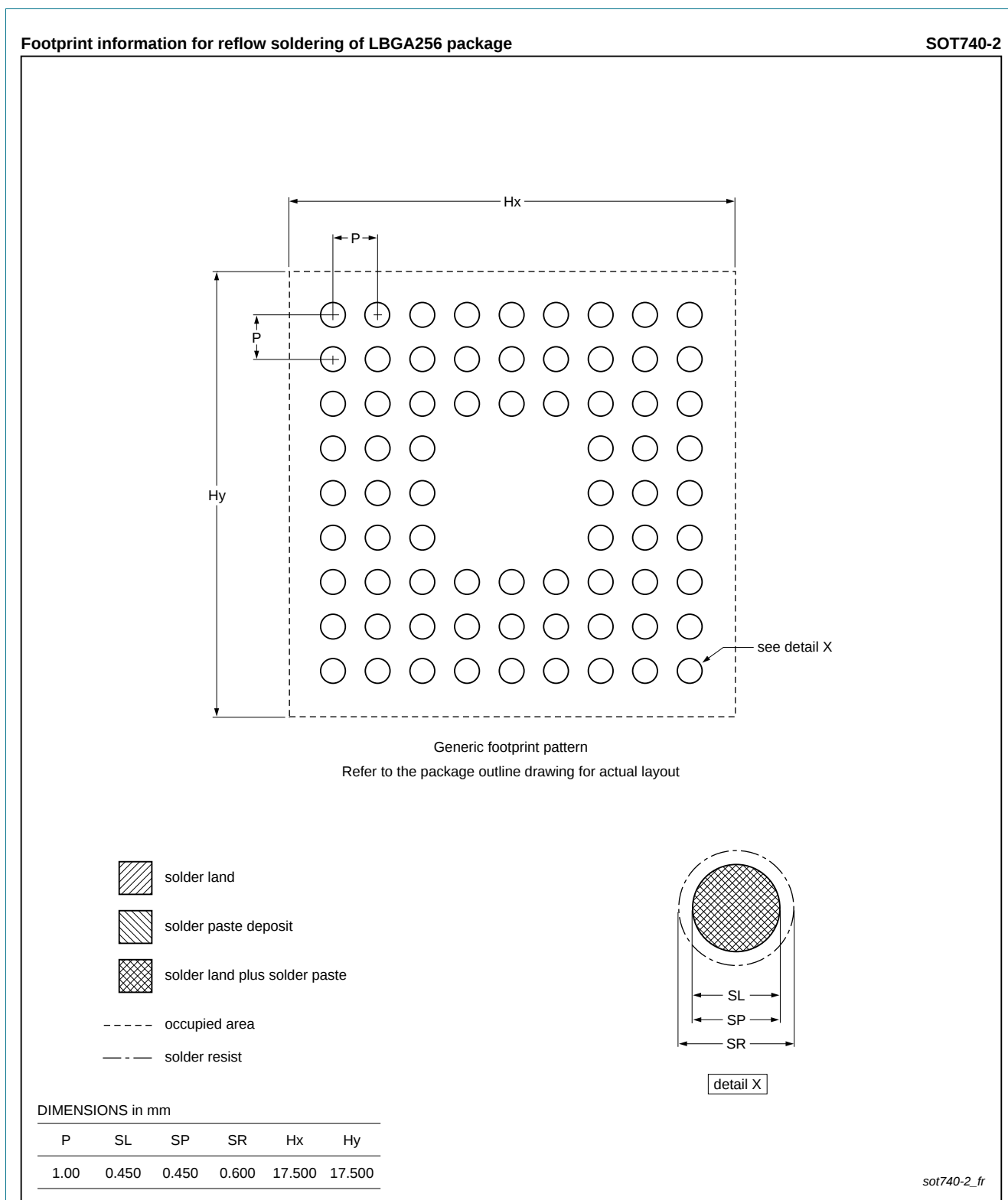
Fig 52. Reflow soldering for the LBGA256 package
