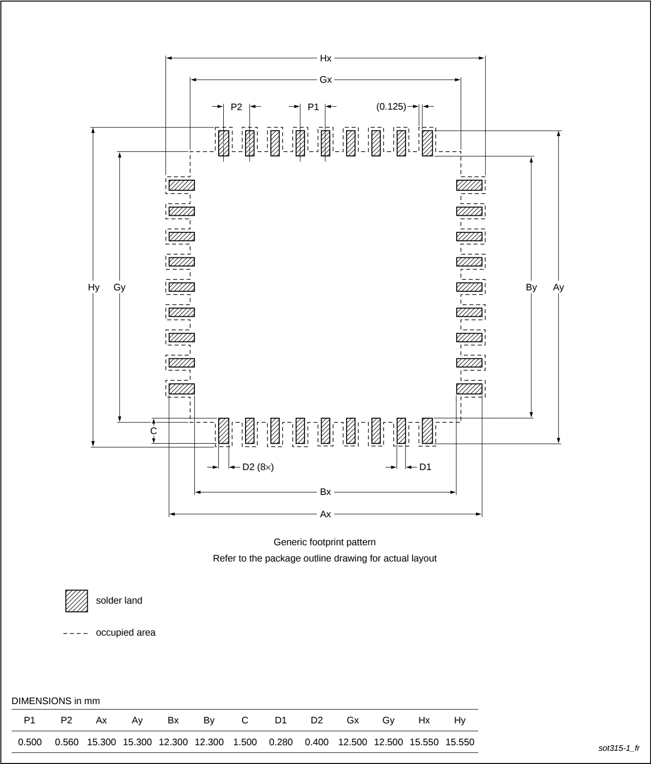
Footprint information for reflow soldering of LQFP80 package SOT315-1
