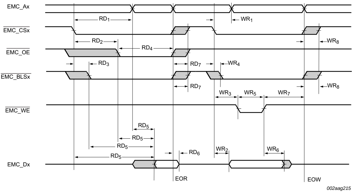
Fig 20. External static memory read/write access (PB =1)
