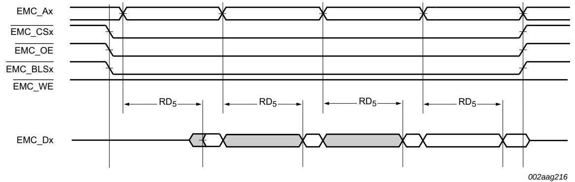
Fig 21. External static memory burst read cycle
