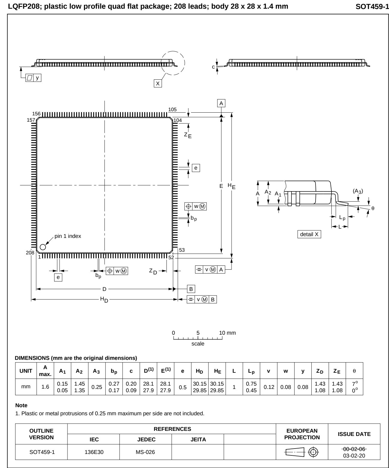
Fig 45. Package outline SOT459-1 (LQFP208)
