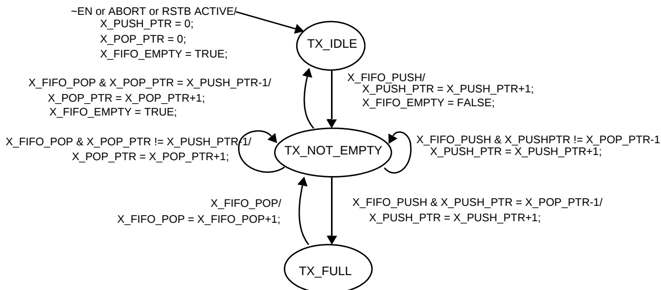
Figure 22. State Diagram of Transmit FIFO
